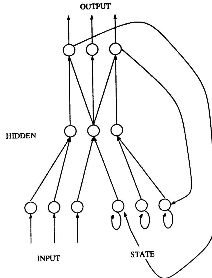
Figure 1. Architecture used by Jordan (1986). Connections from output to state units are one-for-one, with a fixed weight of 1.0. Not all connections are shown.
